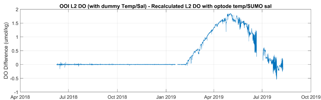
Figure 2: Difference between oxygen values calculated using dummy temp/salinity value and recalculated oxygen values using optode temperature and salinity for SUMO CTD for Deployment 5 NSIF Aanderaa optode.
